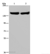
Western Blot analysis of Human placenta and fetal liver tissue using ITGA2B Polyclonal Antibody at dilution of 1:650 Calculated Mw:113kDa
