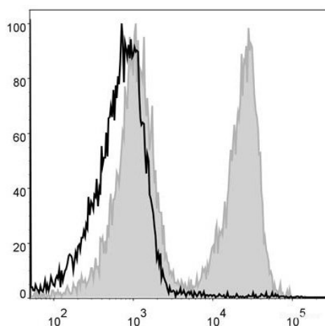
C57BL/6 murine splenocytes are stained with PerCP Anti-Mouse CD3 Antibody (filled gray histogram). Unstained splenocytes (empty black histogram) are used as control.
