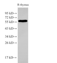
Western Blot analysis of Rat thymus cells using PDCD4 Polyclonal Antibody at dilution of 1:500
