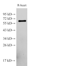
Western Blot analysis of Rat heart cells using PDCD4 Polyclonal Antibody at dilution of 1:500
