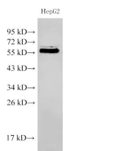
Western Blot analysis of HepG2 cells using PDCD4 Polyclonal Antibody at dilution of 1:500
