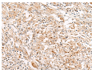
Immunohistochemistry of paraffin-embedded Human liver cancer tissue using FGR Polyclonal Antibody at dilution of 1:35(×200)
