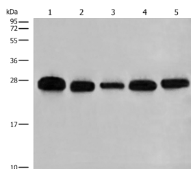
Western blot analysis of 293T A549 HeLa K562 and HEPG2 cell lysates using GATD3B Polyclonal Antibody at dilution of 1:400 Observed Mw:Refer to figures Calculated Mw:28 kDa
