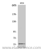
Western Blot analysis of HT29 cells with CHEK1 Polyclonal Antibody Calculated Mw:54kDa
