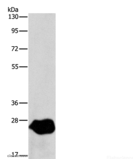
Western Blot analysis of A549 cell using LXN Polyclonal Antibody at dilution of 1:667 Calculated Mw:26kDa
