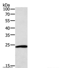
Western Blot analysis of Hela cell using SNAP25 Polyclonal Antibody at dilution of 1:400 Calculated Mw:23kDa
