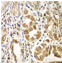
Immunohistochemistry of paraffin-embedded Human gastric using RAC1 Polyclonal Antibody at dilution of 1:100 (40x lens).
